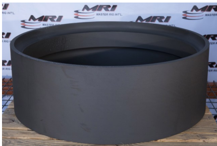
C1 Drawworks High clutch Drum Emsco 6215-0259-00
